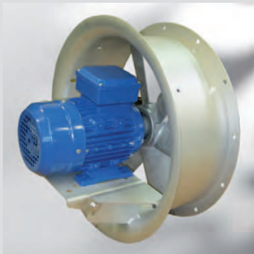
Ventilatori assiali INOX AISI 304 e AISI 316 per basse temperature (Refrigerazione e Alimentare) Axial fans INOX AISI 304 / AISI 316 for low temperatures (Refrigeration and Food processing)
